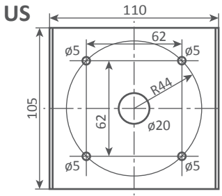
Platine de fixation murale / Wall mounting plate
