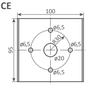
Platine de fixation murale / Wall mounting plate
