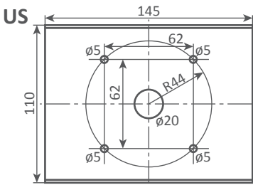
Platine de fixation murale / Wall mounting plate
