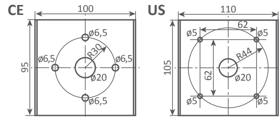
Platine de fixation murale / Wall mounting plate
