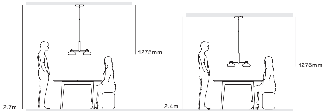
Supplied 30cm tube + add-on 55cm tube- 1275mm overall drop
