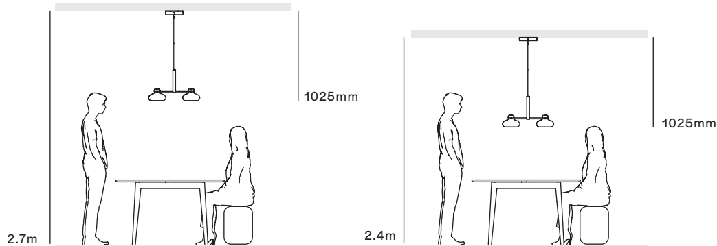
Supplied 30cm tube + add-on 30cm tube - 1025mm overall drop
