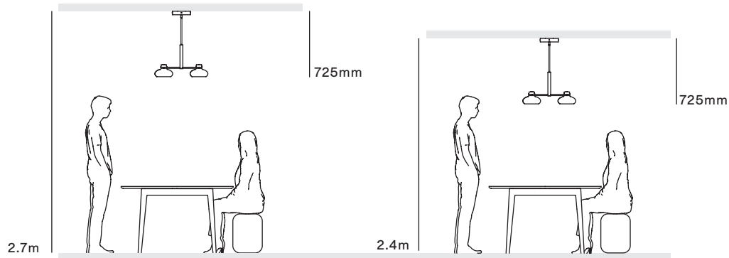
Supplied 30cm tube - 725mm overall drop
