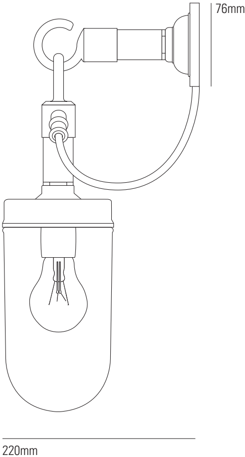
Side View
